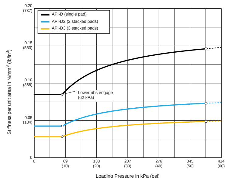
STATIC SECANT STIFFNESS PER UNIT AREA
