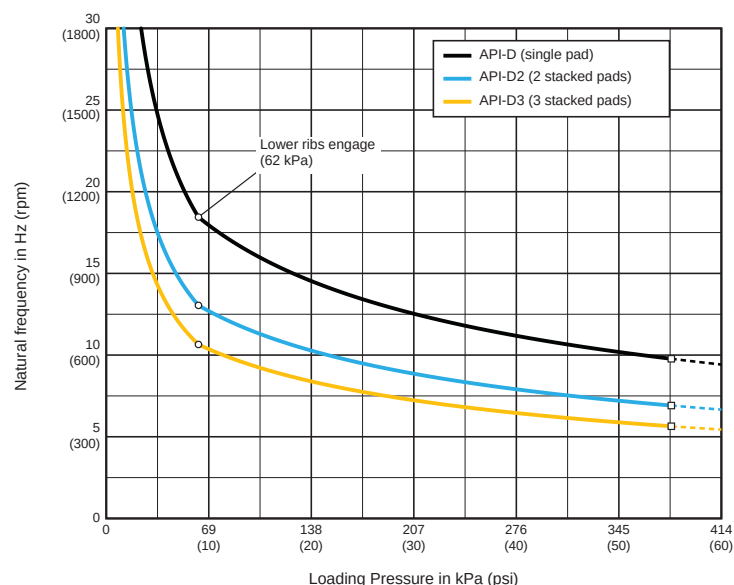
NATURAL FREQUENCY CURVES (estimated from static deflection, per industry practice)
