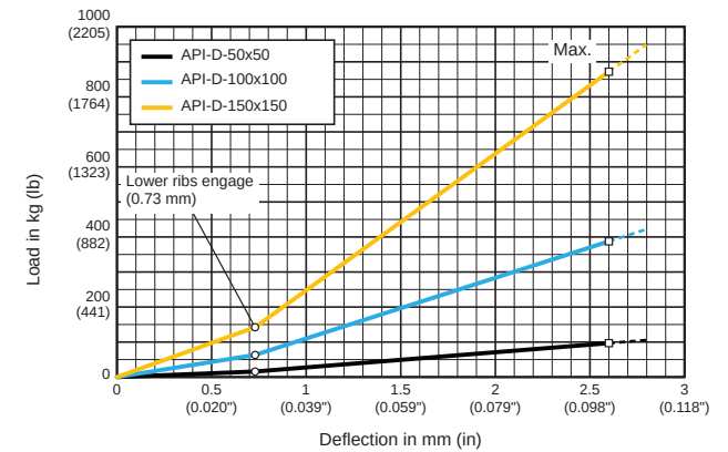
Load - Deflection Graph
